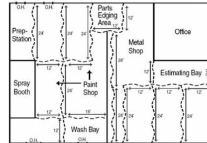
A typical example of Shaver curtain walls in use.
