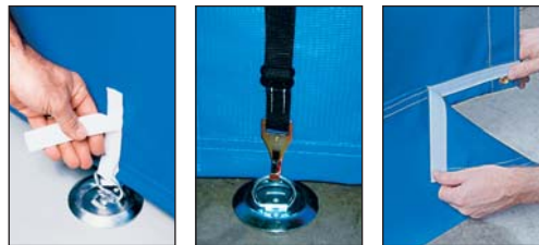
Floor-mounted wind tie "style A"
